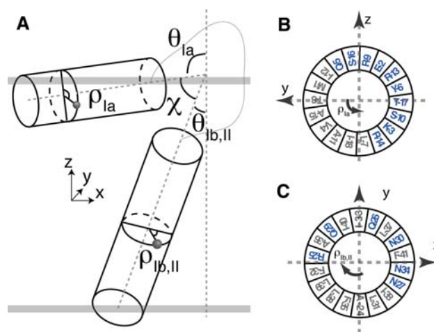
Fig. 2 a Definition of ( \theta , \rho ) describing the orientation of helix with respect to membrane normal Z. ( \theta_{\text{Ib,II}} , \rho_{\text{Ib,II}} ) are the tilt and rotation angles for the domain Ib,II helix, while ( \theta_{\text{Ia}} , \rho_{\text{Ia}} ) are the tilt and rotation angles for the domain Ia helix. The interhelical angle between the two domains is described by \chi . b Helical wheel representation of the reference orientation of domain Ia where \rho_{\text{Ia}} is defined to be zero. The N atom of T8 is aligned to +y axis. \rho_{\text{Ia}} rotates counterclockwise viewing from the top of y-z plane. At \sim 90 degrees, the hydrophilic residues in blue point into bulk solution. c Reference orientation of transmembrane domain where \rho_{\text{Ib,II}} is defined to be zero
