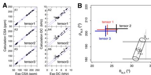
Fig. 6 a Comparison of the experimental and calculated CSA and DC for different values of the CSA tensor components shown in Table 1. The diagonal errors indicate ranges of \pm 5 ppm and \pm 0.5 kHz for CSA and DC, respectively. b Effects of the different CSA tensor components on the tilt and rotation angles for the helix defined by domains Ib and II of PLN. Tensors 1 (Wu et al. 1995), 2 (Page et al. 2008), and 3 are shown in red, black, and blue, respectively
