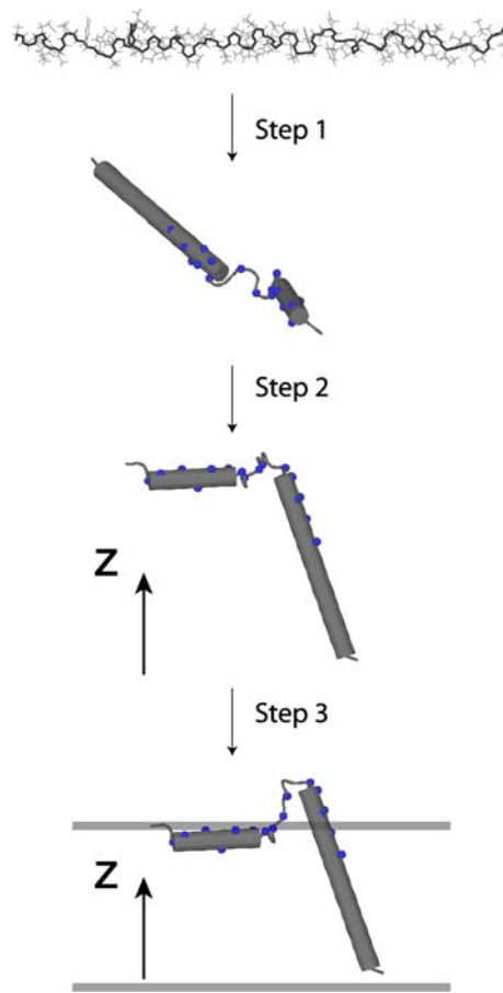
Fig. 1 Overview of the hybrid refinement protocol for the simultaneous determination of structure and topology of membrane proteins. Step 1: Starting from an extended structure, the simulated annealing protocol minimizes a target function containing only solution NMR data (NOEs, torsion angles, and hydrogen bonds). Step 2: The orientational constraints derived from solid-state NMR are included together with solution NMR restraints to obtain the correct orientation along the Z direction. Step 3: Depth of insertion is determined using rigid body minimization in the presence of the depth of insertion potential, keeping the helical orientation with respect to Z fixed. The resulting structural ensemble is refined using low temperature simulated annealing
