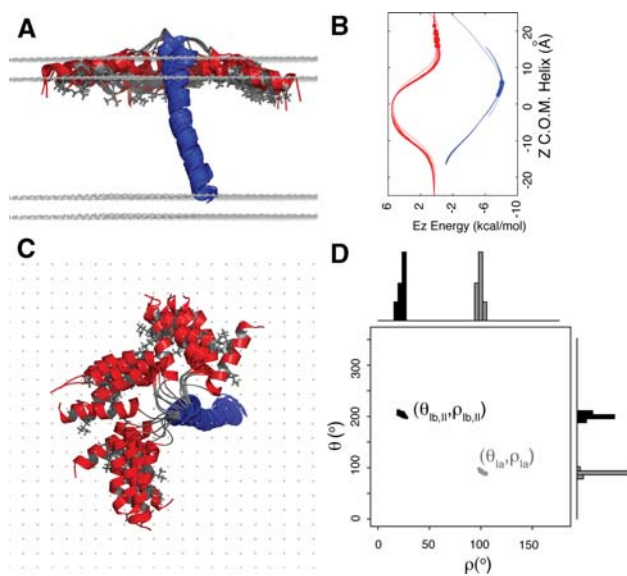
Fig. 5 a Conformational ensemble (structures and topologies) representing the 20 lowest energy structures in the virtual bilayer. Domain Ia is colored in red, and domains Ib and II are in blue. Hydrophobic side chains of domain Ia are shown in grey. Structure overlay is performed by rotating along Z and translating along X and Y, resulting in no changes in E_z energy and PISEMA data. b Position of the cytoplasmic and transmembrane domains with respect to the depth of insertion E_z potential. c Top view of a . d Distribution of \theta and \rho angles in the final structural ensemble
