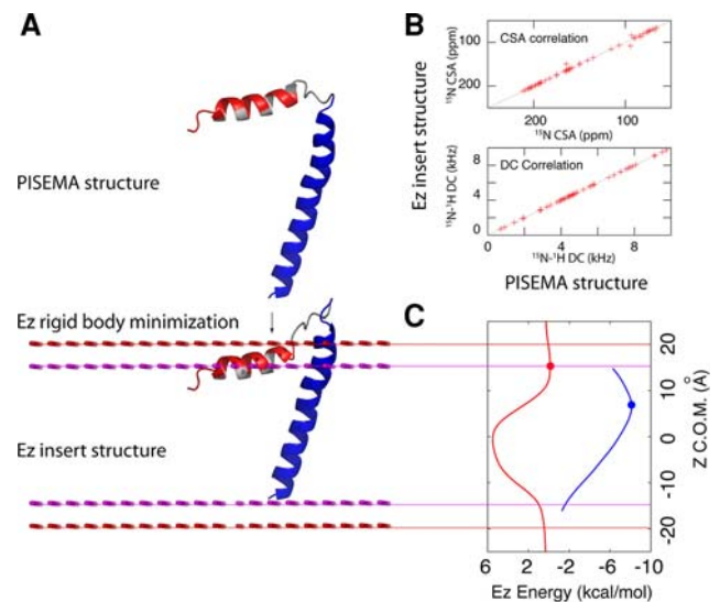
Fig. 4 Rigid-body minimization using the knowledge-based E_z potential. a Backbone cartoon representation of a selected PLN conformer before ( upper panel ) and after rigid-body minimization. b Comparison of the simulated CSA and DC before and after E_z minimization. The only discrepancies are due to residues located in the dynamic loop, which do not have CSA and DC restraints. c Representation of the E_z potential energy function for the domain Ib, II ( blue ) and domain Ia ( red ) helices. After minimization, both domains reside in the minima
