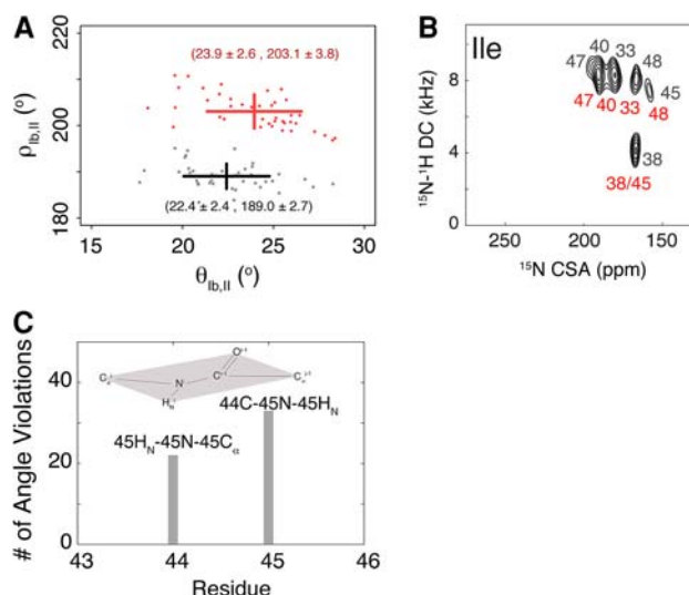
Fig. 7 Effects of the resonance misassignment on the calculation of the structural topology of PLN. a Plots of the distribution of the rotation angles for the two ensembles obtained from simulated annealing calculations. The correct assignments give rise to an average rotation angle of 203^\circ , while the incorrect assignment gives rise to an average rotation angle of 189^\circ . b Experimental PISEMA spectra with the two equiprobable assignments for the isoleucine residues of PLN derived from the combinatorial assignment procedures (see text). c Histogram representing the number of violations obtained for residues 44 and 45 in the conformational ensemble generated with the incorrect assignments
