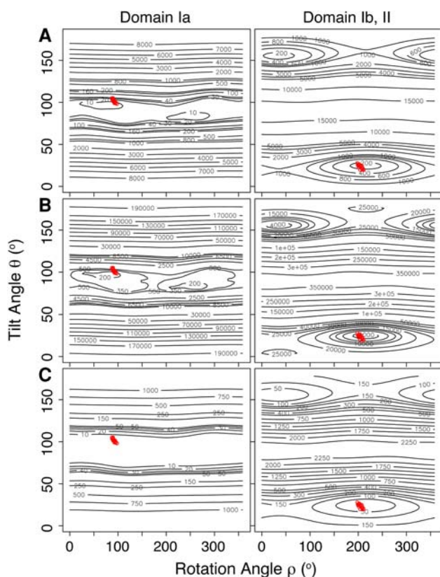
Fig. 8 Projection of (\theta, \rho) of the hybrid ensemble (20 lowest) for the two helical domains of PLN onto the PISEMA potential surfaces obtained using rigid helix fitting. Three different scoring functions are used to generate the potential surfaces: a \text{score}_1 = \text{RMSD}_{\text{DC}} + \text{RMSD}_{\text{CSA}} \times \frac{\text{DC}_{\text{max}}}{\text{CSA}_{\text{max}}} , b \text{score}_2 = \text{RMSD}_{\text{DC}} \times \frac{\text{CSA}_{\text{max}}}{\text{DC}_{\text{max}}} + \text{RMSD}_{\text{CSA}} and c \text{score}_3 = \frac{\text{RMSD}_{\text{DC}}}{\text{DC}_{\text{max}} - \text{DC}_{\text{min}}} + \frac{\text{RMSD}_{\text{CSA}}}{\text{CSA}_{\text{max}} - \text{CSA}_{\text{min}}} . These plots demonstrated that the topologies derived from the hybrid method correspond to the lowest energy minima identified in all of the PISEMA potential surfaces
